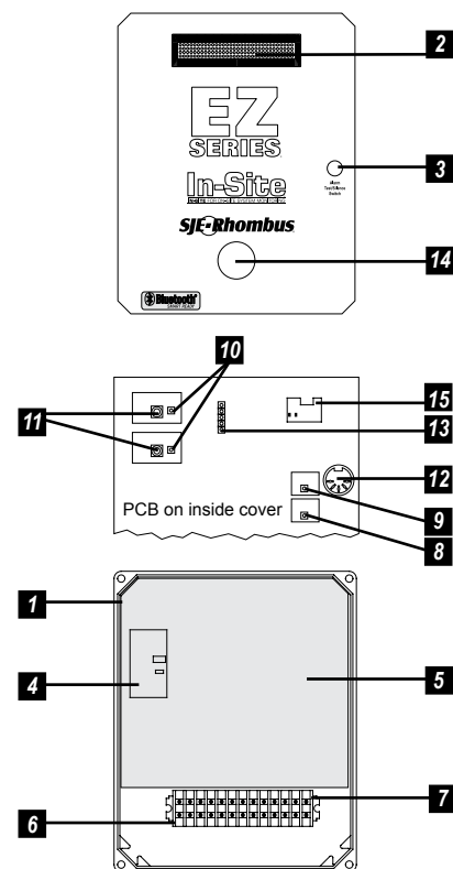
Model Shown EZIS1W114C3A4A6A10E24E30A
