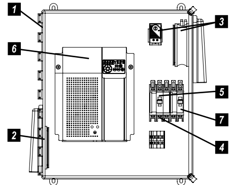
VARIOspeed® 3R (240V model)
